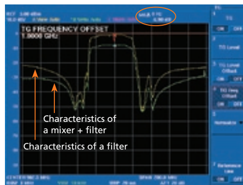
Measurement of mixer frequency conversion loss characteristics
