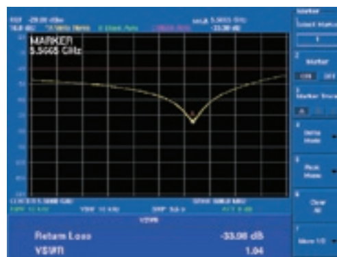
Filter return loss measurement
