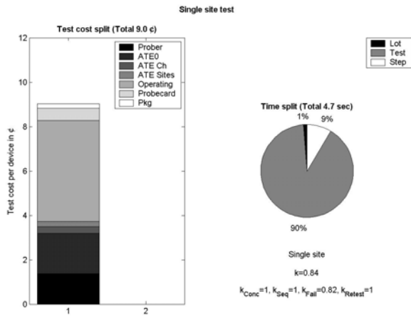
Figure 3: Test Cost Split for Single Site Test
