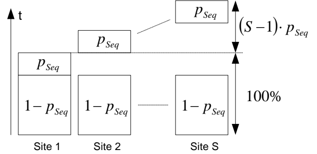
Figure 2: Partially Sequential Multi-Site Test
