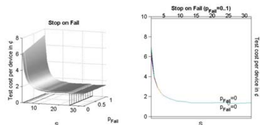
Figure 15: Minimum Sensitivity of 'Stop on Fail'
