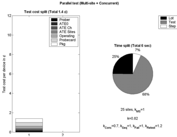
Figure 11: Lowest Test Cost with Parallel Test
