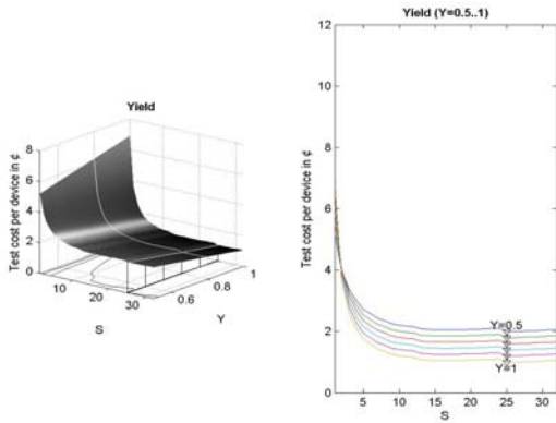
Figure 16: Yield has No Influence on Best Number of Sites
