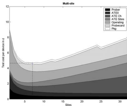
Figure 4: Multi-Site Reduces Test Cost by \approx 50\%
