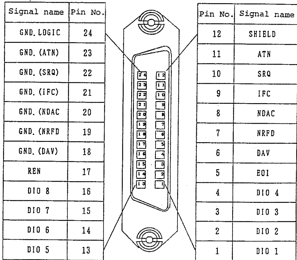
Figure 5 - 2 GPIB Connector
