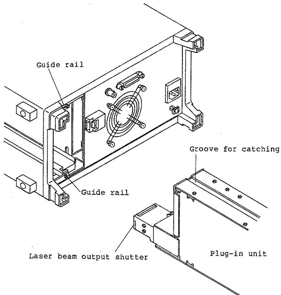
Figure 1 - 5 Mounting and Dismounting the Plug-in Unit
