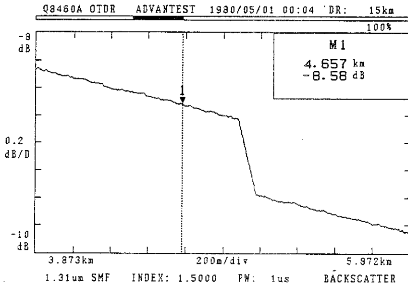
Figure 3 - 3 After Averaging
