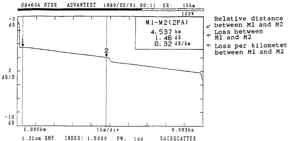
Figure 3 - 17 Measurement Display of Loss
