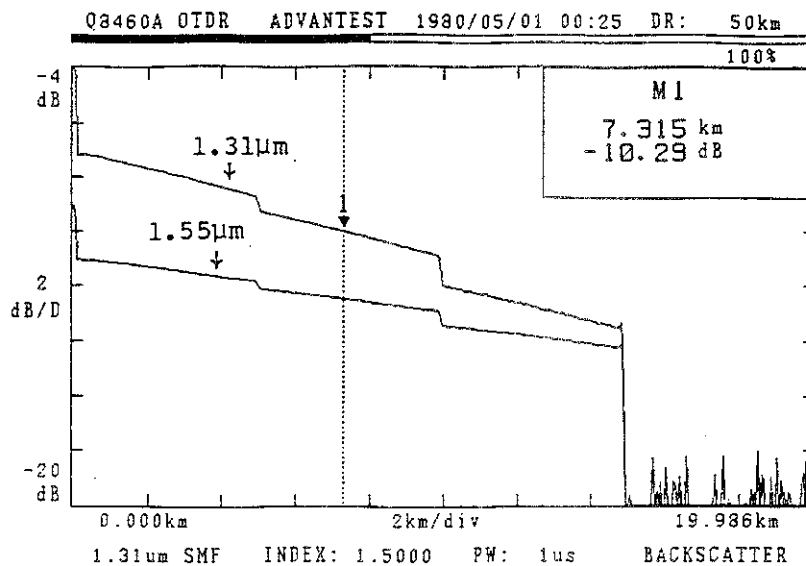
Figure 3 - 29 Two Waveforms Simultaneous Comparison by SAVE/VIEW Function
