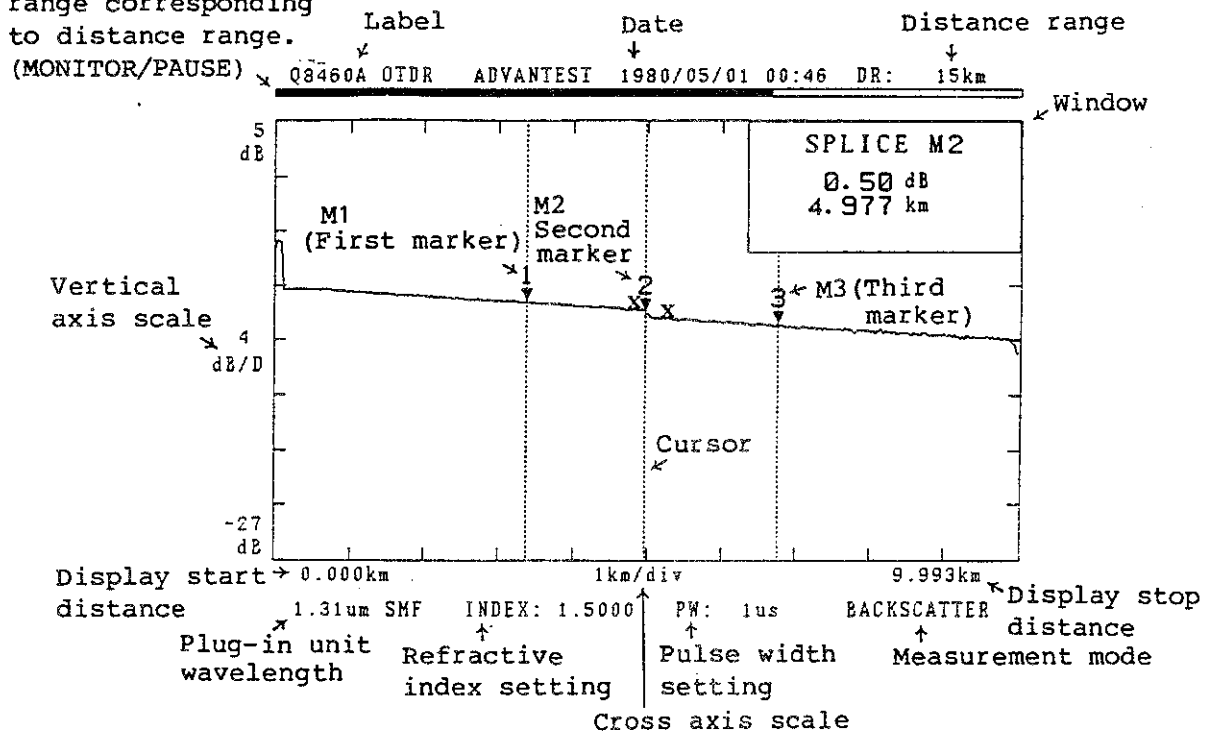
Figure 2 - 1 CRT Display
