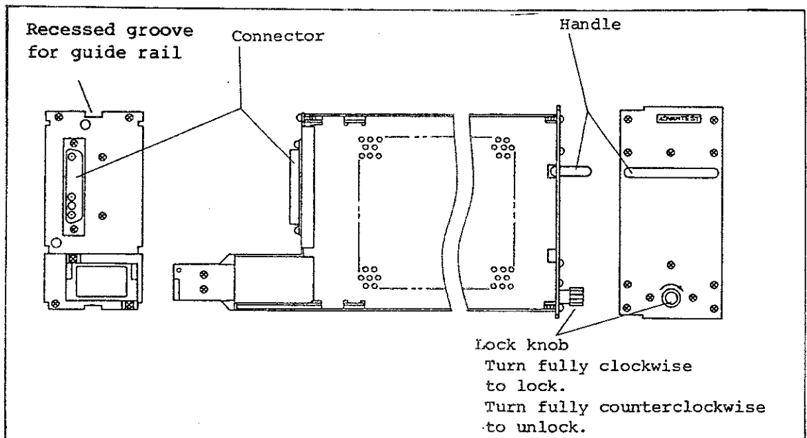
Figure 1 - 4 Plug-in Unit
