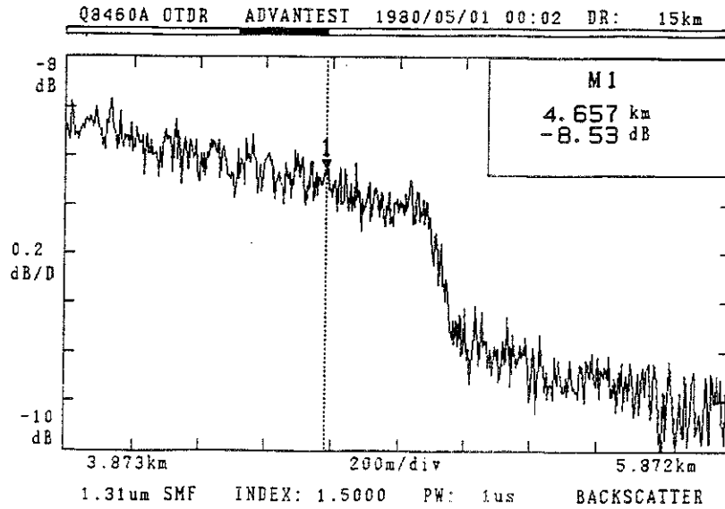
Figure 3 - 2 Before Averaging
