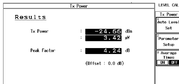
Figure 2-1 2 GHz Modulation Signal Measurement Sample (Using the 3GPP2 Level Calibration Function)
