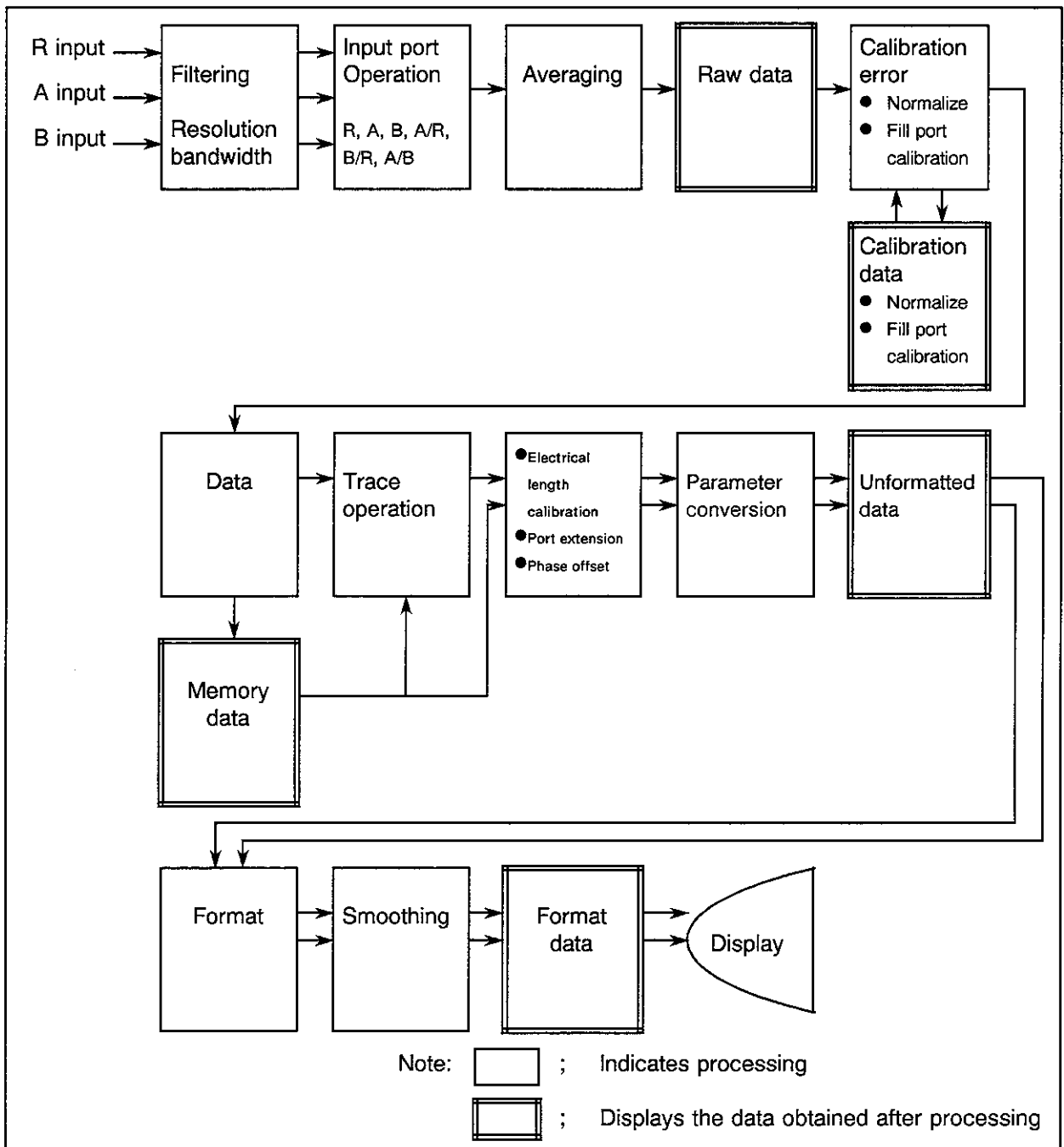
Figure 1-2 Data Flowchart
