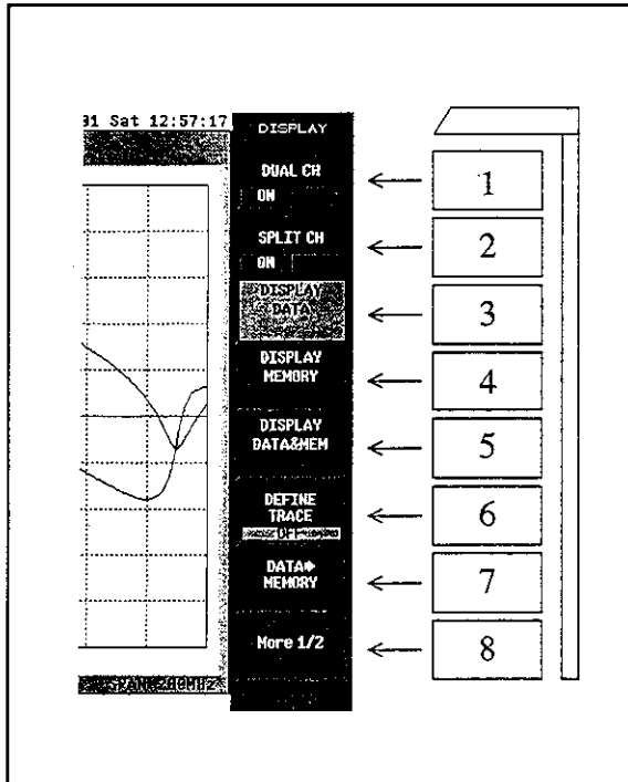
Figure 3-1 Software key
