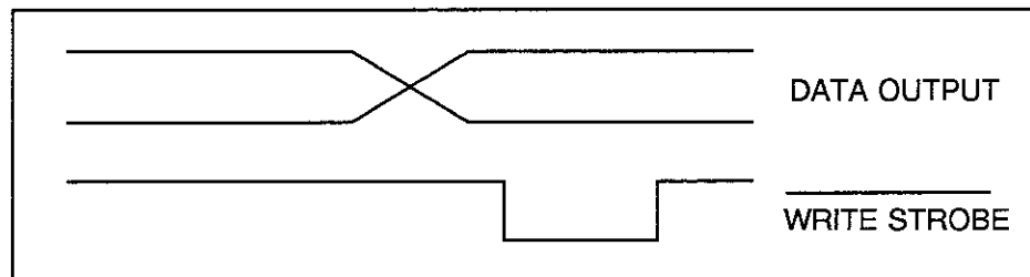
Figure 4-6 Timing Chart of WRITE STROBE
