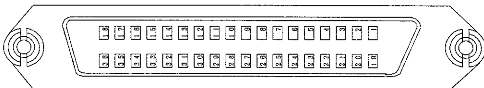
Figure 4-7 36-pin Connector Internal Pin Assignment and Signal
