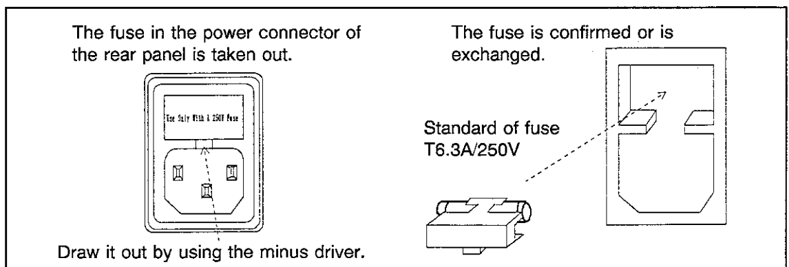
Figure 1-4 Confirmation and exchange of fuses
