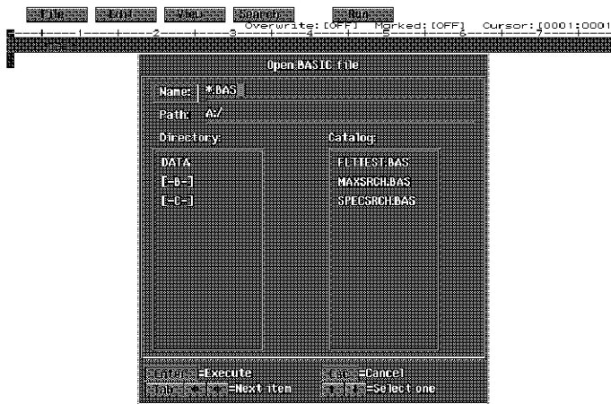
Figure 3-3 Dialog Box for the Open ... Command
