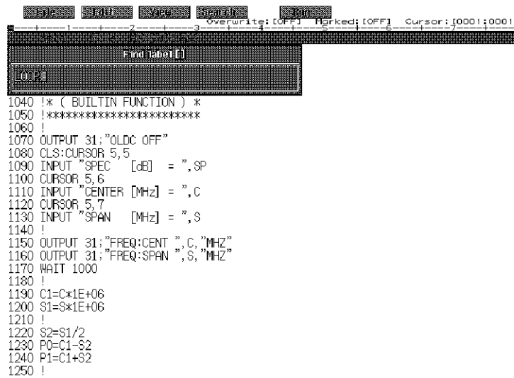
Figure 8-3 Dialog Box of Find label ... Command
