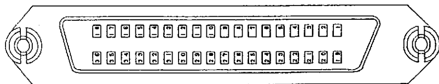
Figure 5-2 36-pin Connector Internal Pin Addignment and Signal
